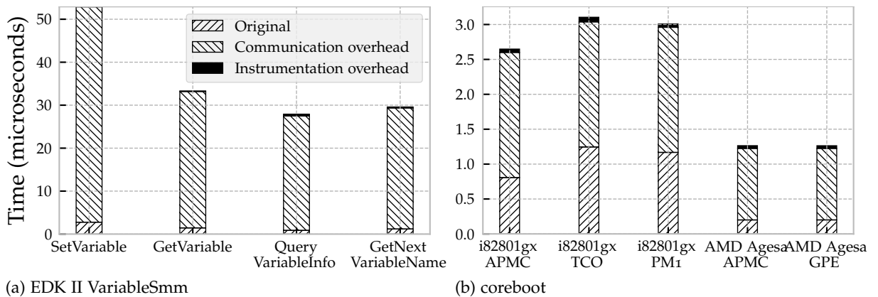
Figure 12.1: Time (in microseconds) to execute each SMI handler (averaged over 100 executions) with the original time, and the overhead divided between the communication overhead due to pushing packets to the FIFO and the instrumentation overhead
